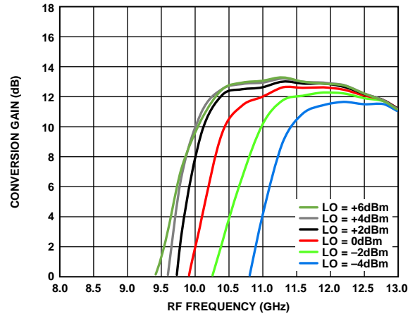
Figure 31. Conversion Gain vs. RF Frequency at Various LO Powers, T A = 25°C
