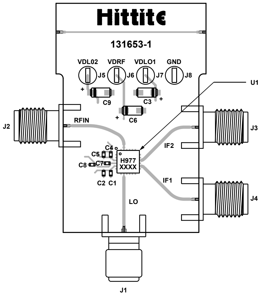
Figure 53. Evaluation PCB
