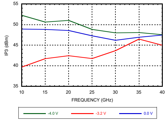
Input IP3 vs. Frequency @ 10dBm Vctrl2 = Variable, Vctrl1 = 0V
