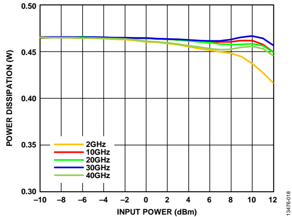
Figure 18. Power Dissipation at 85°C
