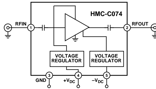
Figure 2. Pin Configuration
