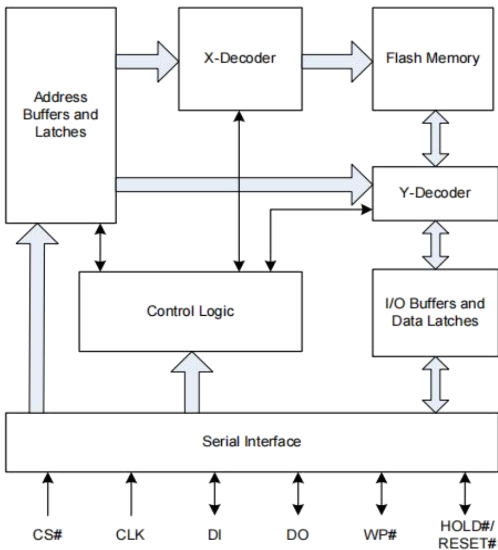
Figure 4.1 Block Diagram
