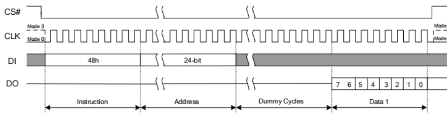
Figure 9.35 Read Security Registers Instruction
