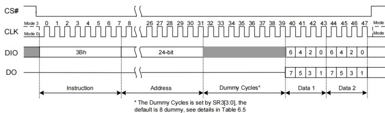
Figure 9.15 Fast Read Dual Output Instruction Sequence Diagram
