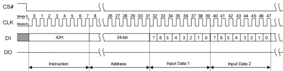
Figure 9.34 Program Security Registers Instruction
