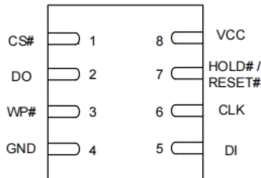
Figure 5.2 4 x 4mm DFN
