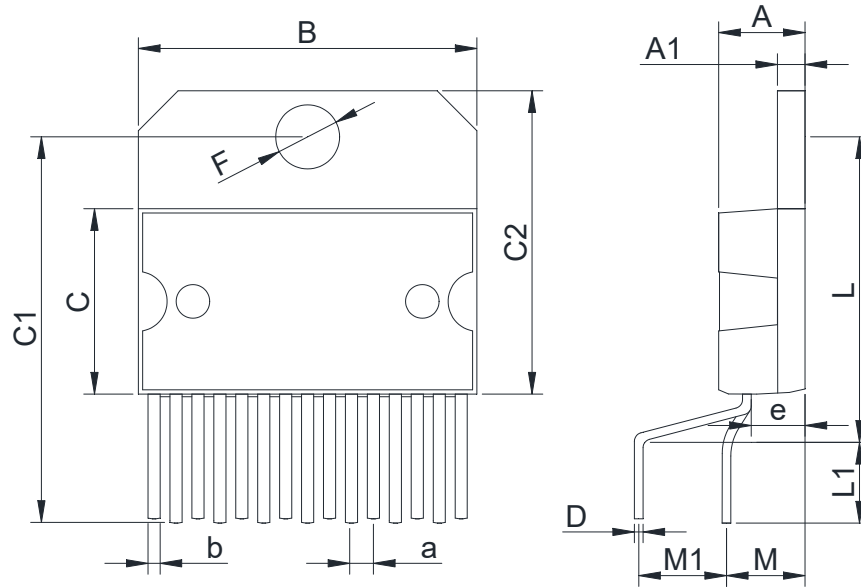
Dimensions In Millimeters(Multiwatt15)
