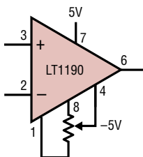
INPUT OFFSET VOLTAGE CAN BE ADJUSTED OVER A \pm 150\text{mV} RANGE WITH A 1\text{k}\Omega TO 10\text{k}\Omega POTENTIOMETER
