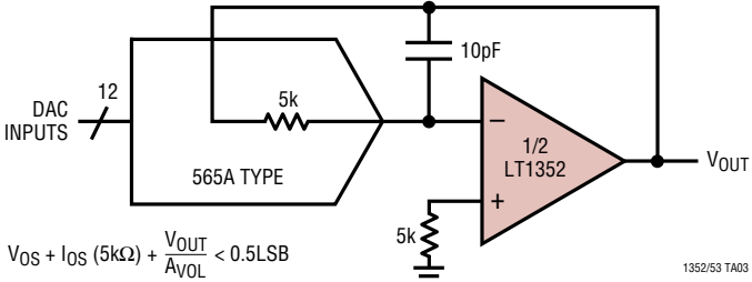
DAC I-to-V Converter
