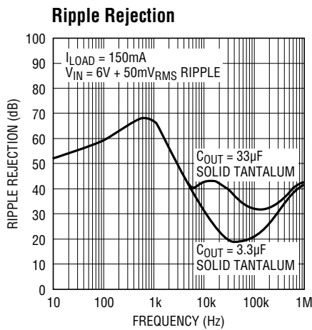
LT1521 • TPC31
