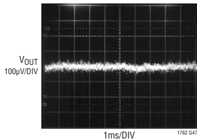
LT1762-5 10Hz to 100kHz Output Noise C_{BYP} = 0.01\mu F
