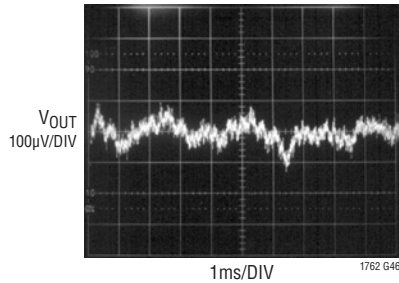
LT1762-5 10Hz to 100kHz Output Noise C_{BYP} = 1000pF
