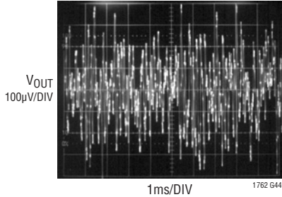
LT1762-5 10Hz to 100kHz Output Noise C_{BYP} = 0
