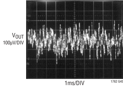
LT1762-5 10Hz to 100kHz Output Noise C_{BYP} = 100pF
