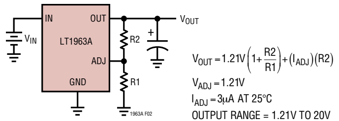
Figure 2. Adjustable Operation
