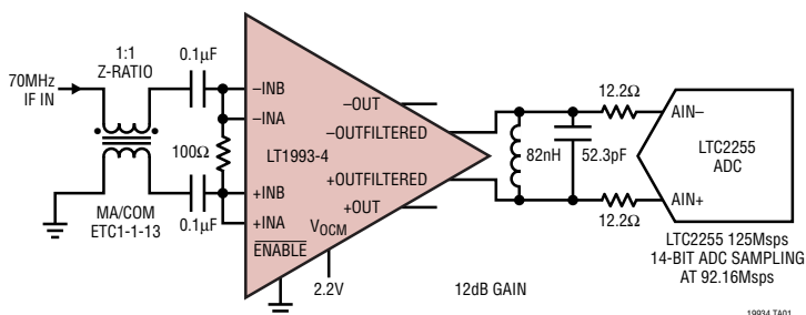
ADC Driver with Single-Ended to Differential Conversion
