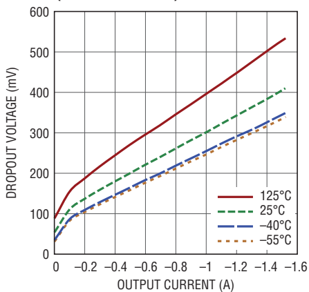
Typical Dropout Voltage (DD-PAK/T0-220)
