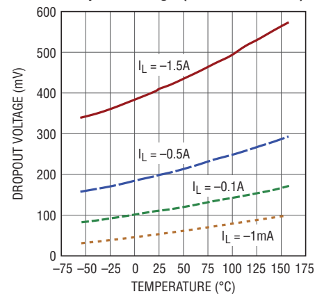
Dropout Voltage (DD-PAK/T0-220)
