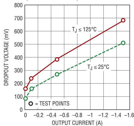
Guaranteed Dropout Voltage (DD-PAK/T0-220)
