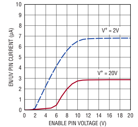
Enable Pin Current
