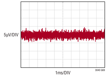
Output Noise: 10Hz to 100kHz
