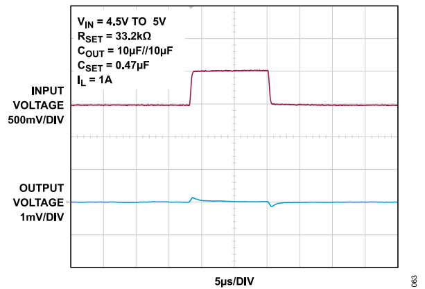
Figure 63. Line-Transient Response
