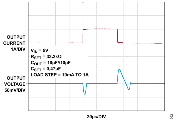
Figure 62. Load-Transient Response
