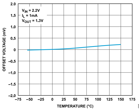
Figure 6. Offset Voltage ( V_{OUT} - V_{SET} ) vs. Temperature
