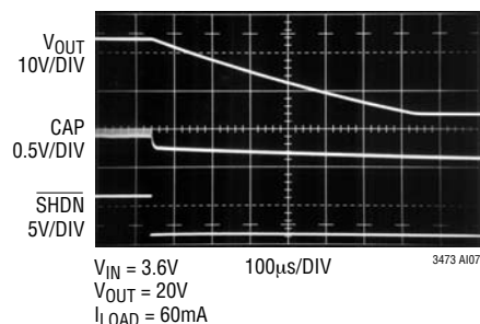
Shutdown Waveforms
