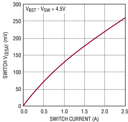
Switch V_{\text{CESAT}}
