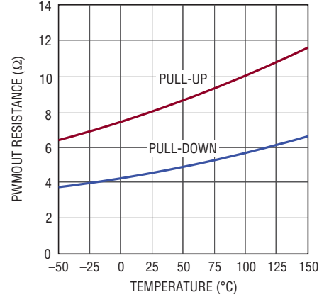
PWMOUT On-Resistance vs Temperature
