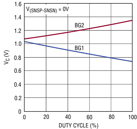
V_C Voltage vs Duty Cycle
