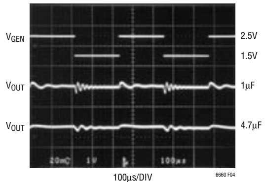
Figure 4. I_{OUT} = 1mA
