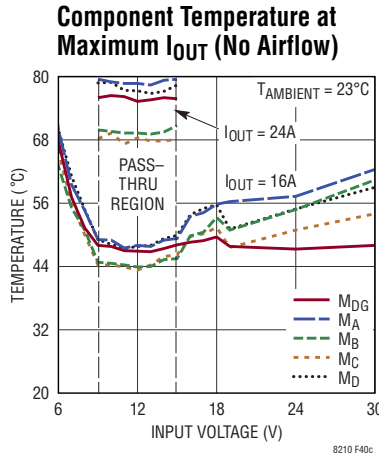
Figure 40. 24A/16A, 8V to 16V Pass-Thru Regulator
