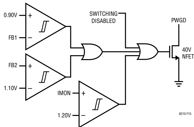
Figure 15. PWGD Logic
