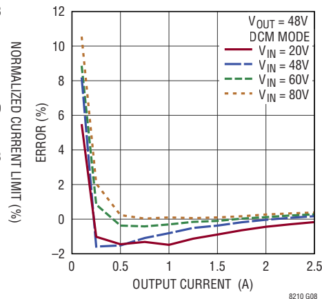
IMON Measurement Accuracy (Figure 37)
