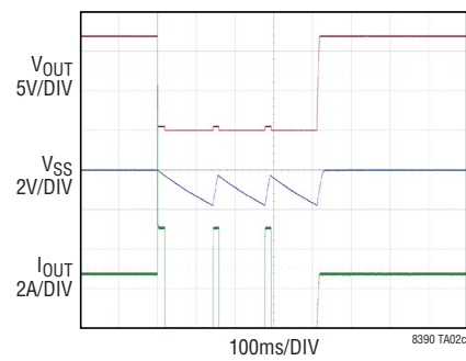
Output Short Protection ( V_{IN} = 12V , I_{OUT} = 3A )
