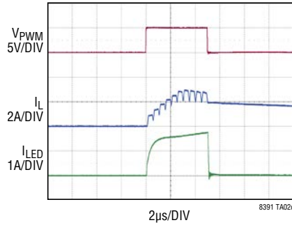
100Hz 2000:1 External PWM Dimming ( V_{IN} = 18V )
