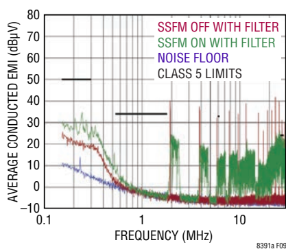
Figure 9. CISPR 25 Average Conducted EMI
