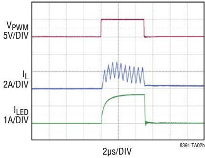
100Hz 2000:1 External PWM Dimming ( V_{IN} = 32V )
