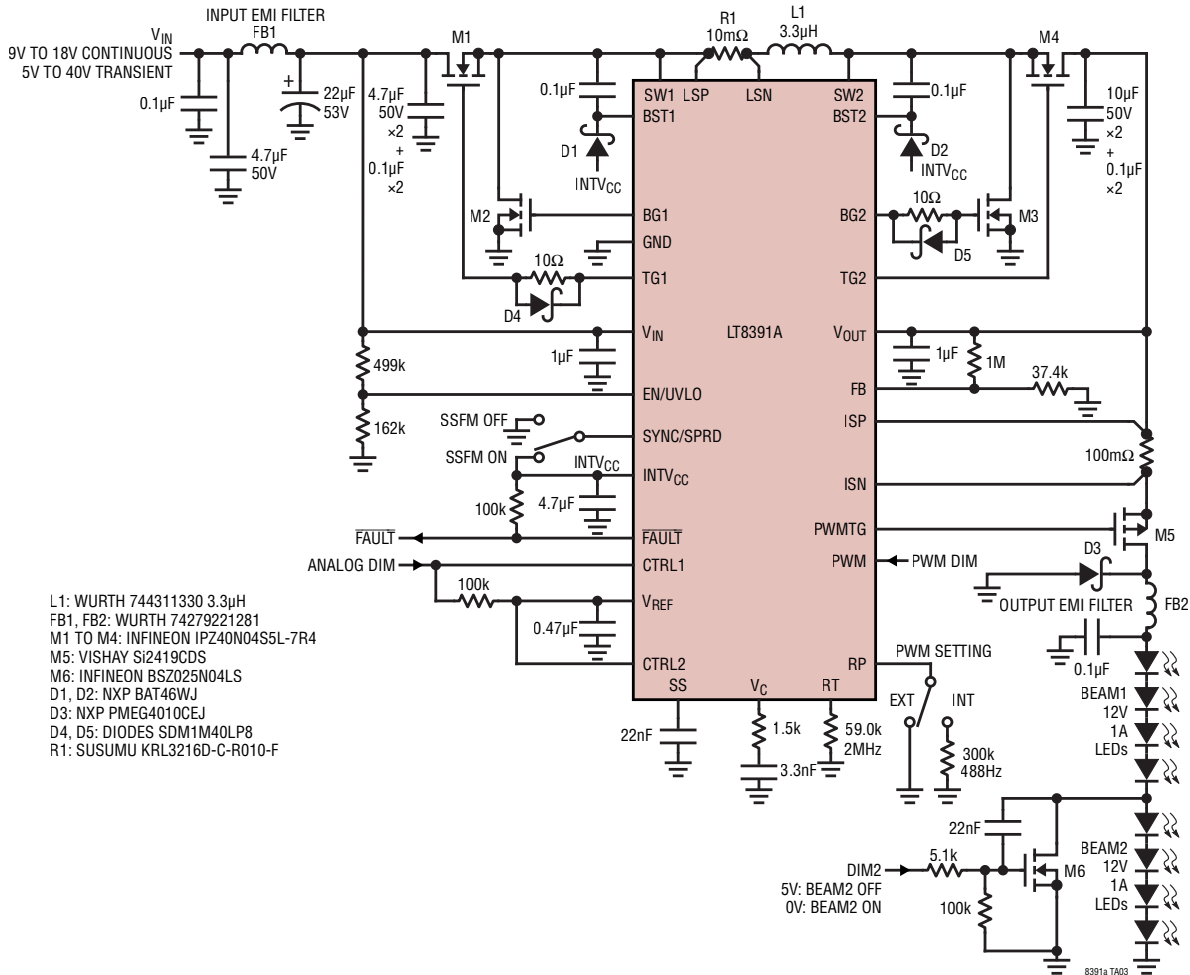
Low EMI 2MHz Buck-Boost Driving 2-Beam LEDs (2× 12V, 1A)
