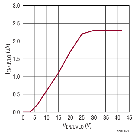
EN/UVLO Current vs Voltage
