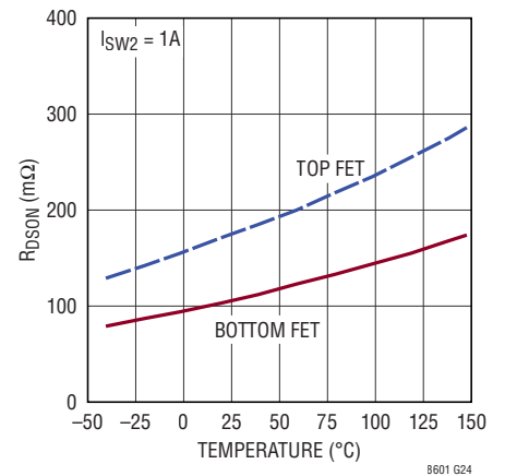
Channel 2 R DS(ON) vs Temperature
