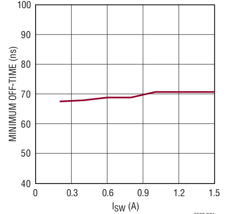
Channel 3/Channel 4 Minimum Off-Time vs I_{SW}
