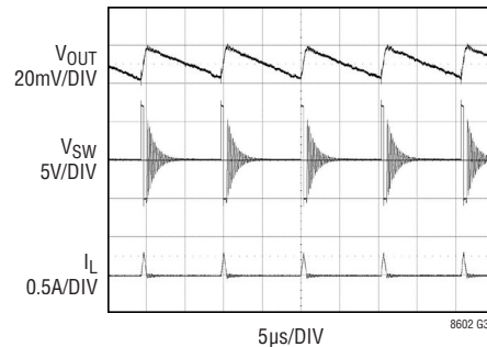
Light Load Waveforms
