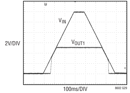
Channel 1 Start-Up and Dropout, R_L = 20\Omega
