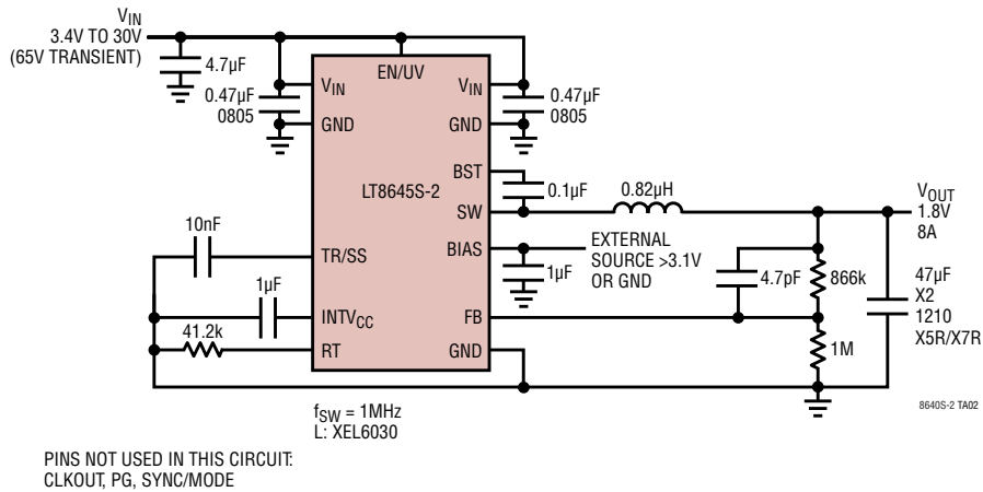
1.8V, 8A Step-Down Converter
