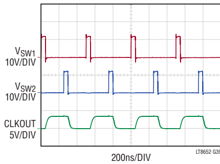
CH1, CH2 and CLKOUT Two-Phase Operation
