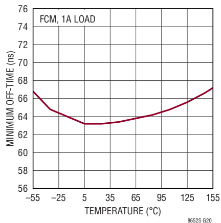
Minimum Off-Time
