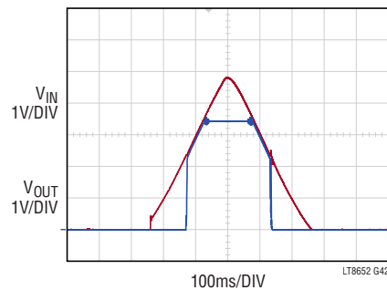
Start-Up Dropout Performance Burst Mode Operation
