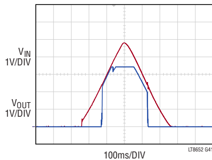
Start-Up Dropout Performance Forced Continuous Mode
