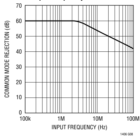
Input Common Mode Rejection vs Input Frequency
