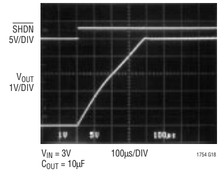
Start-Up Time
