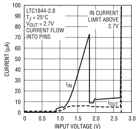
1844 F08 Figure 8. Reverse Current vs Input Voltage
