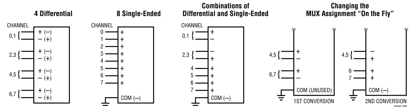
Figure 8. Examples of Multiplexer Options on the LTC1854/LTC1855/LTC1856
