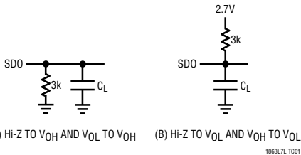
Load Circuits for Access Timing
