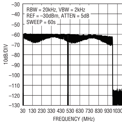
157 Carrier DOCSIS Gap Channel Wideband ACLR, f_{DAC} = 2.7Gps
