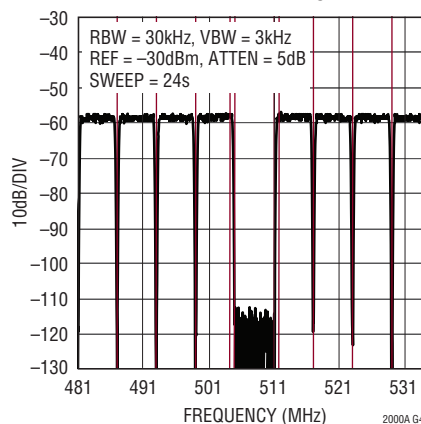
157 Carrier DOCSIS Gap Channel Narrowband ACLR, f_{DAC} = 2.7Gps
