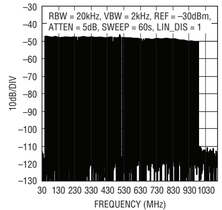
157 Carrier Tones with Gap Channel Wideband ACLR, f_{DAC} = 2.7Gps
