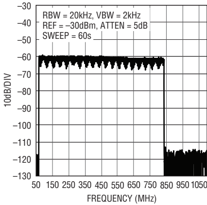
128 Carrier DOCSIS Low Band Wideband ACLR, f_{DAC} = 2.7Gps
