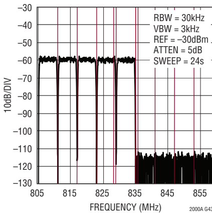
128 Carrier DOCSIS Low Band Narrowband ACLR, f_{DAC} = 2.7Gps
