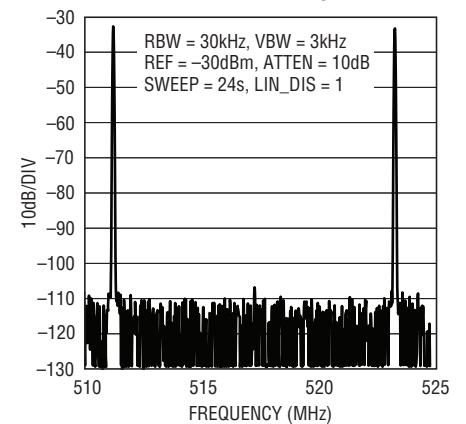
157 Carrier Tones with Gap Channel Narrowband ACLR, f_{DAC} = 2.7Gps
