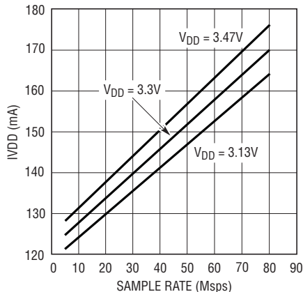
LTC2204: I_{DD} vs Sample Rate, f_{IN} = 5.1\text{MHz} , \text{dBFS} , DITH = 0, RAND = 0
