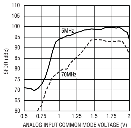
LTC2216 SFDR vs Analog Input Common Mode Voltage, 5MHz and 70MHz, -1\text{dBFS}
