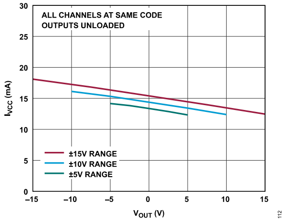
Figure 12. I_{VCC} vs. V_{OUT}
