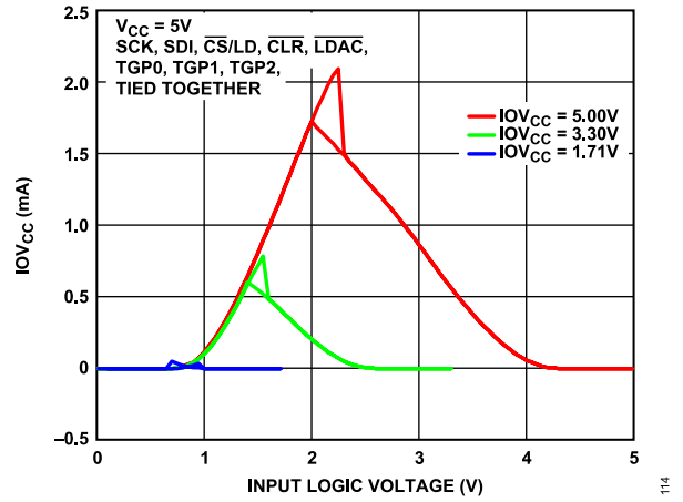
Figure 14. IOV_{CC} vs. Input Logic Voltage
