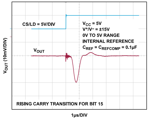
Figure 15. Glitch Impulse
