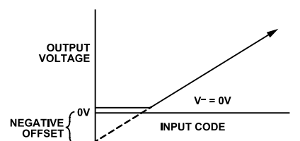
Figure 53. Effects of 0 V to 5 V Output Range for Single-Supply Operation, Overall Transfer Function
