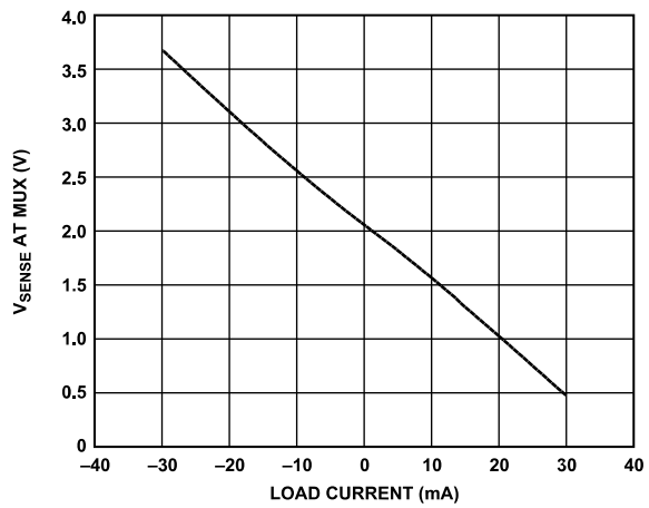
Figure 20. V_{SENSE} at MUX vs. Load Current
