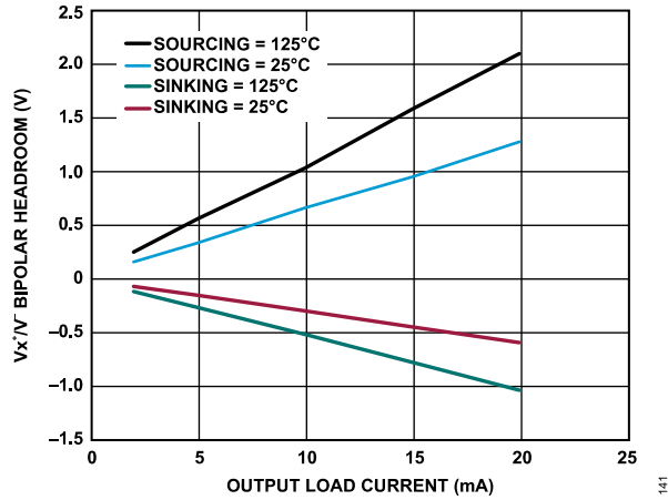
Figure 40. V_{x^+}/V^- Bipolar Headroom vs. Output Load Current
