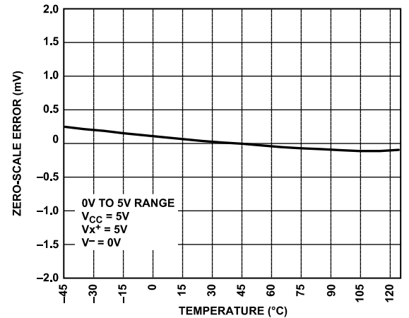
Figure 6. Zero-Scale Error (ZSE) vs. Temperature
