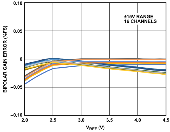
Figure 4. Gain Error vs. V_{REF}
