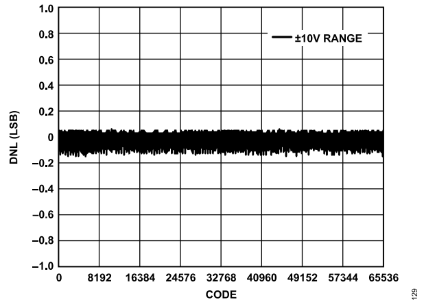
Figure 26. DNL vs. Code
