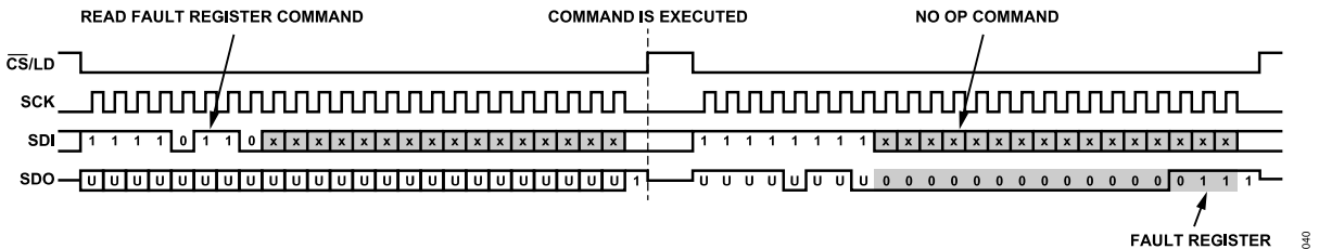
Figure 45. Typical Read Command Sequence for 24-Bit Words
