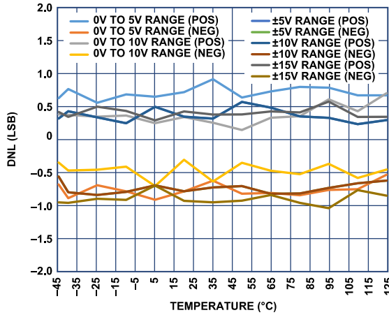
Figure 28. DNL vs. Temperature
