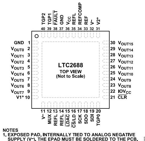
Figure 3. Pin Configuration
