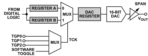
Figure 47. Toggle Operation
