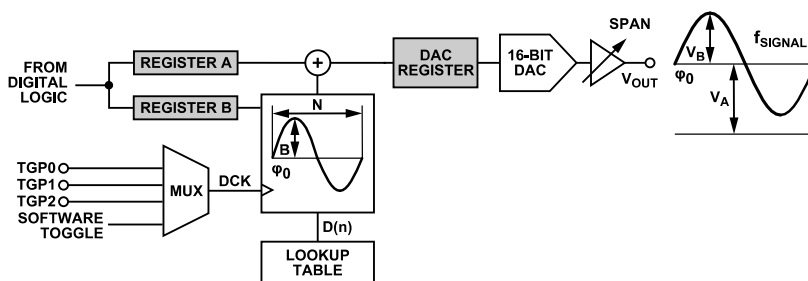
Figure 49. Dither Signal Operation
