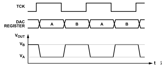
Figure 48. TCK Timing
