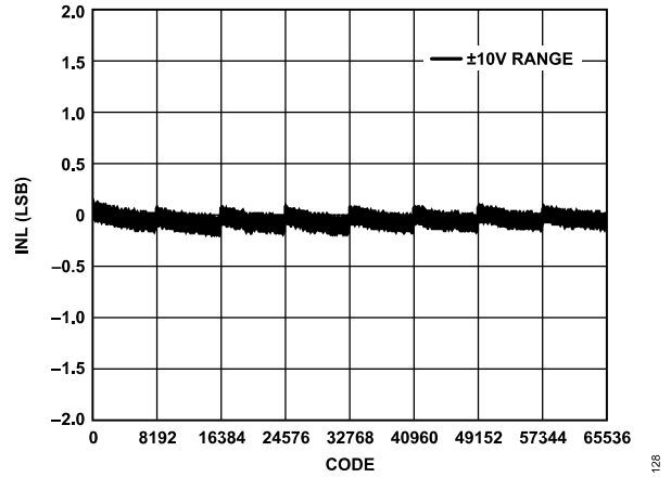
Figure 25. INL vs. Code
