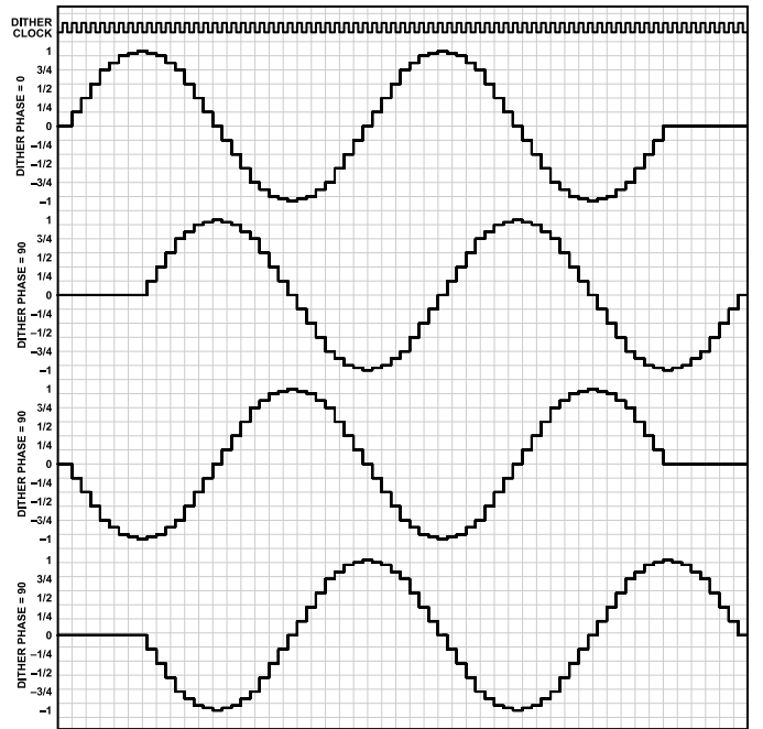
Figure 51. Sinusoidal Waveforms for Various Values of \phi_0
