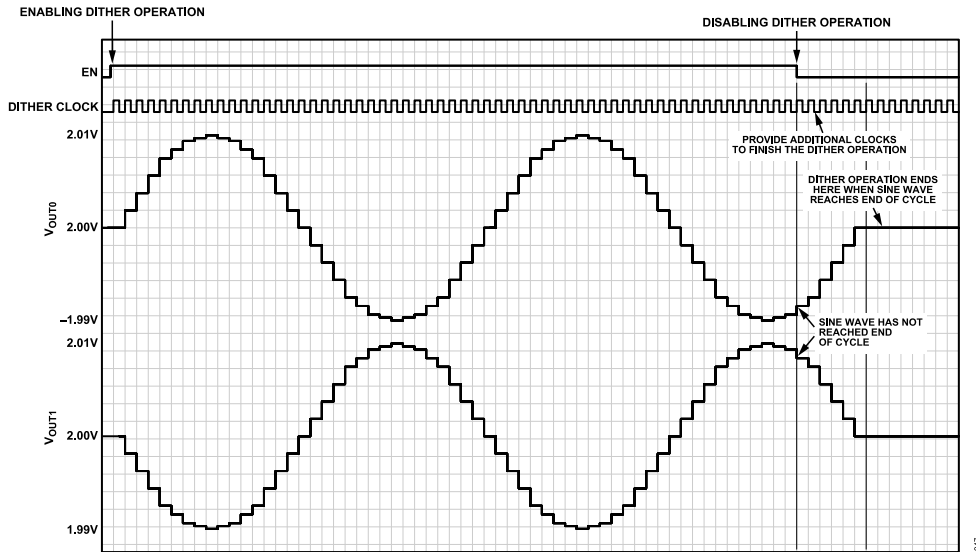
Figure 52. Termination of Sinusoidal Dither Waveforms
