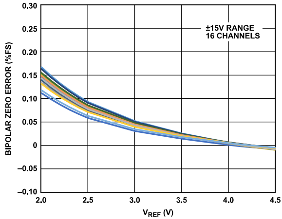
Figure 5. Bipolar Zero Error vs. V_{REF}
