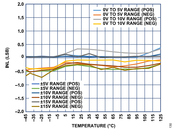
Figure 27. INL vs. Temperature
