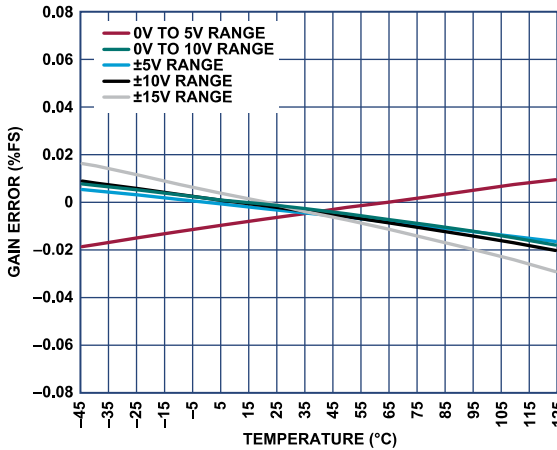
Figure 29. Gain Error vs. Temperature
