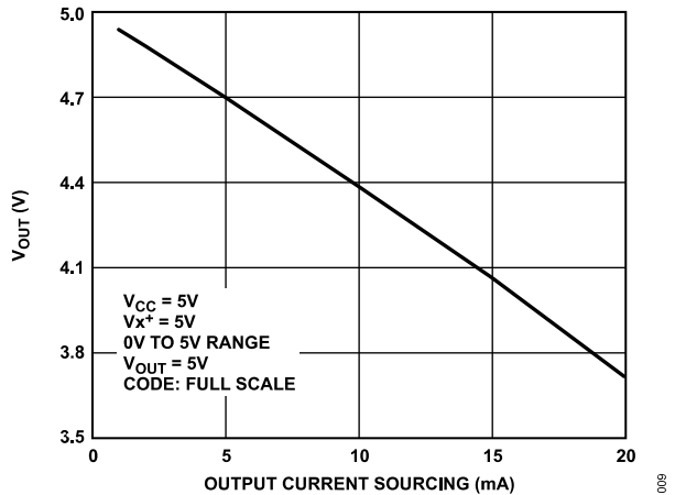
Figure 9. V_{OUT} vs. Output Current Sourcing
