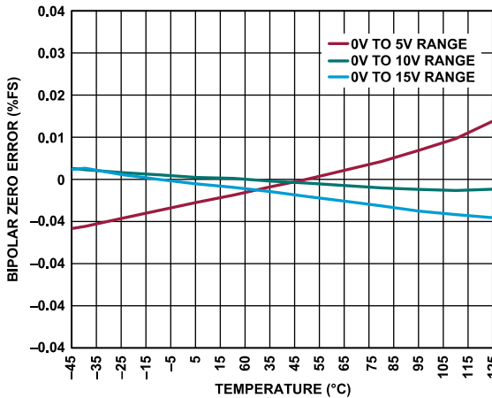
Figure 30. Bipolar Zero Error vs. Temperature
