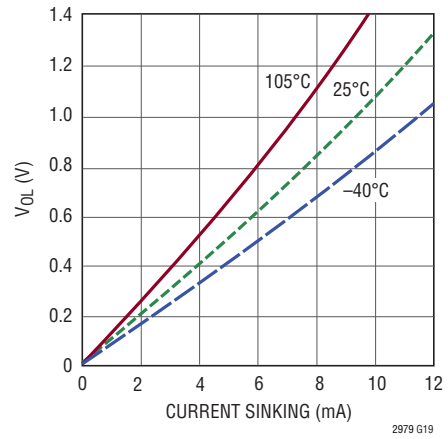
V_{OUT\_EN[3:0]} and V_{IN\_EN} Output V_{OL} vs Current
