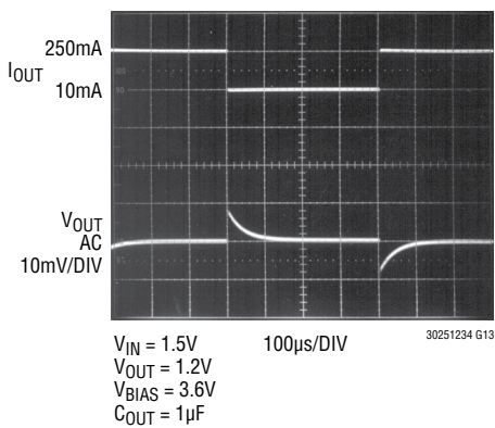
Transient Response
