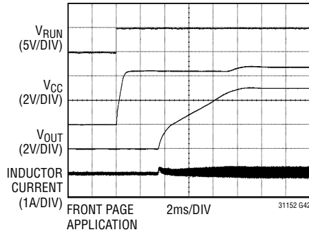
Soft-Start Waveforms
