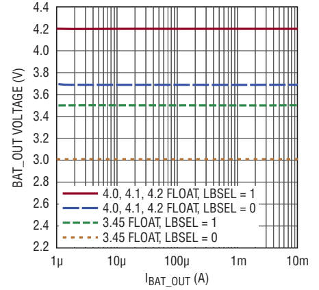
Battery Connect Voltage at BAT_OUT vs I_{\text{BAT\_OUT}}
