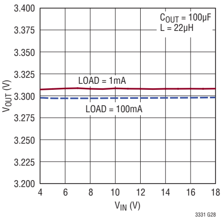
Buck Line Regulation, 3.3V
