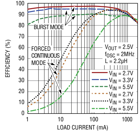
2A Buck Efficiency vs I_{LOAD} , V_{OUT} = 2.5\text{V}
