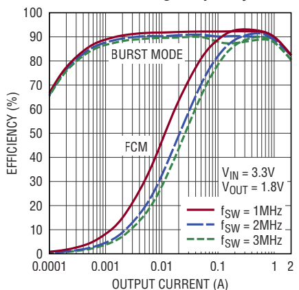
2A Buck Efficiency vs Output Current Across Switching Frequency
