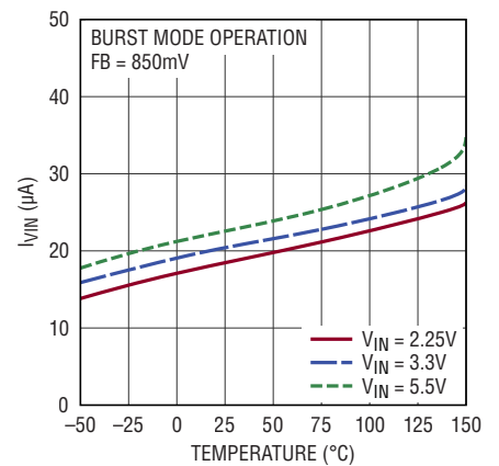
Buck V_{IN} Quiescent Current vs Temperature
