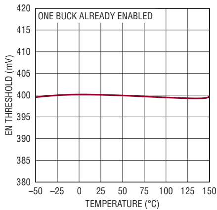
EN Pin Rising Threshold vs Temperature
