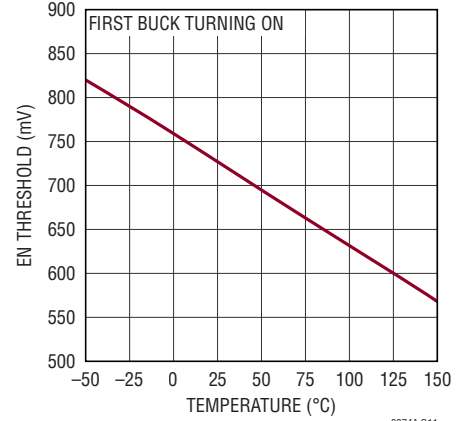
EN Pin Rising Threshold vs Temperature
