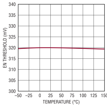
EN Pin Falling Threshold vs Temperature
