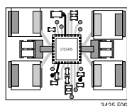
Figure 6. Example Board Layout for a 10W, 4-Phase Boost Converter. Total Area = 0.50in 2 (with All Components Mounted on the Topside of Board)
