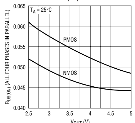
Effective R_{DS(ON)}
