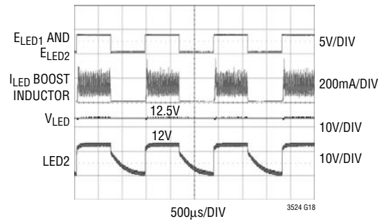
LED Burst Dimming Waveforms LED2 and VLED
