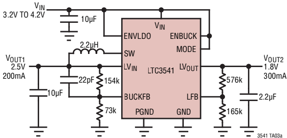
Dual Output with Minimal External Components Using Auto Start-Up Sequence, Buck in Pulse Skip Mode for Low Noise Operation
